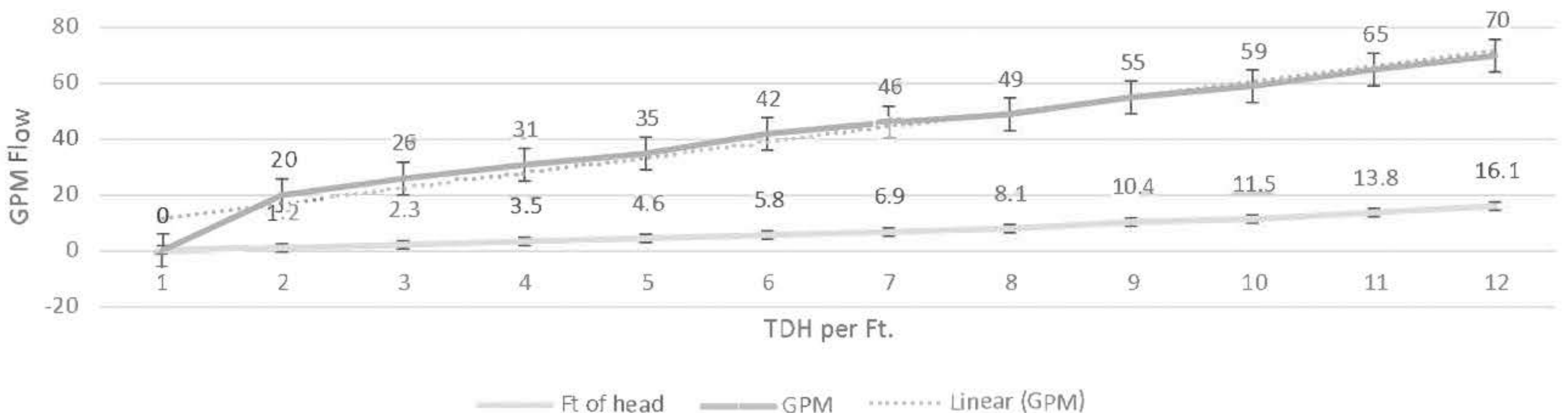
Head Loss
